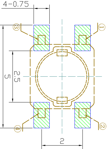
P.C.B MOUNTING PATTERN DIMENSION the following soldering are recommended for reflow soldering
